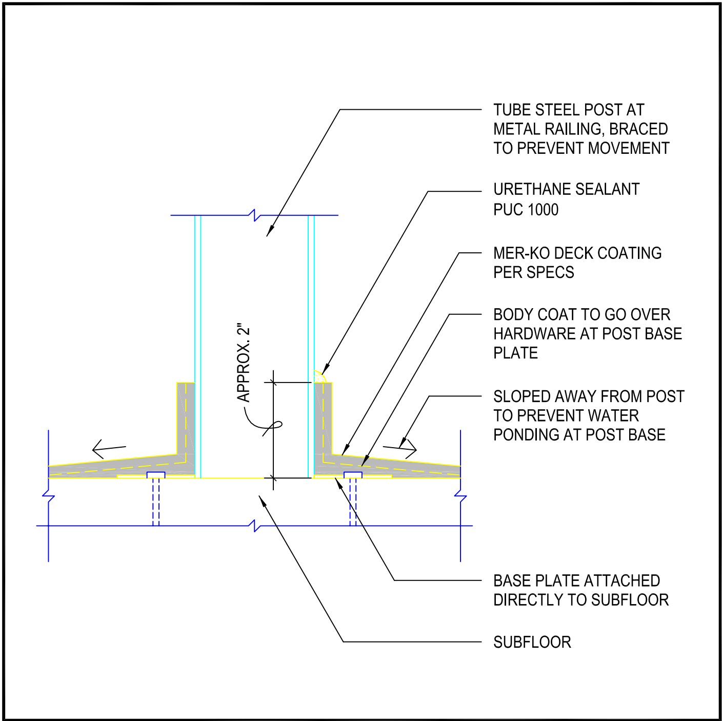
TUBE STEEL RAIL DETAIL
