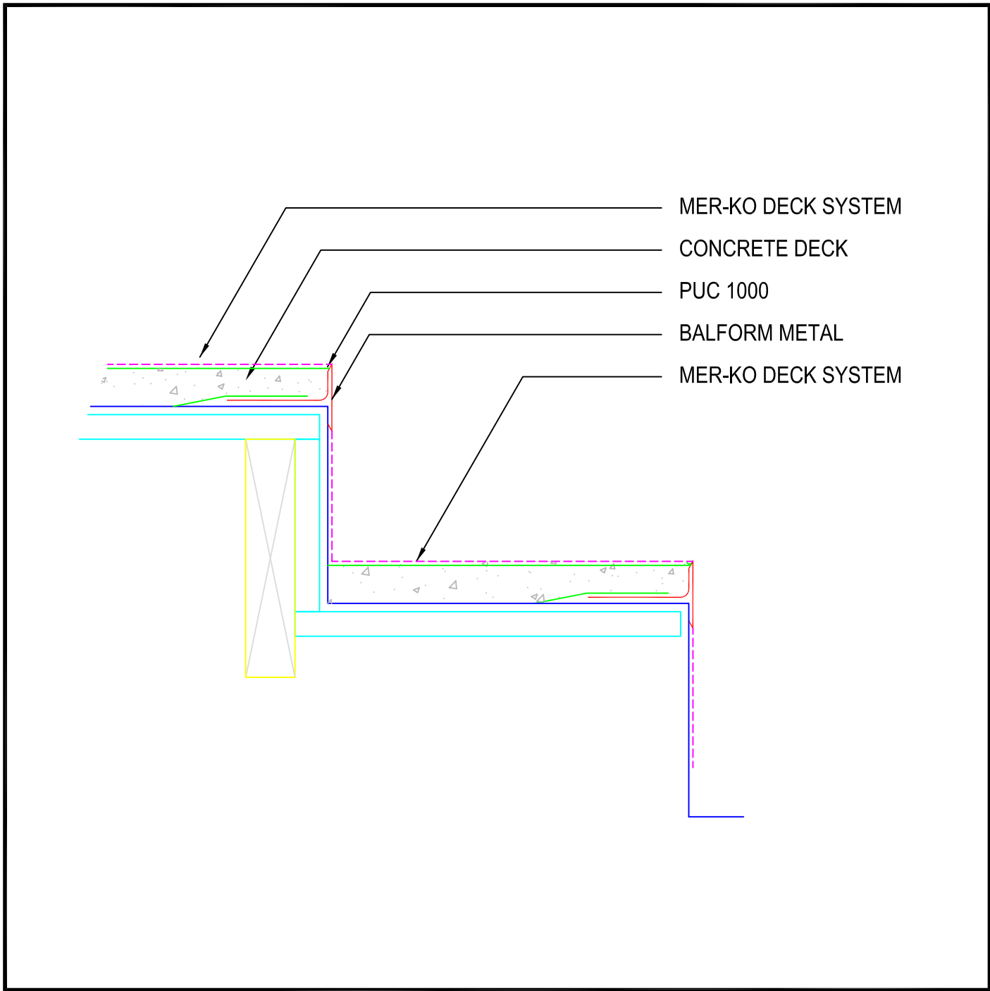
DECKING OVER CONCRETE STAIRS WITH METAL BALFORM
